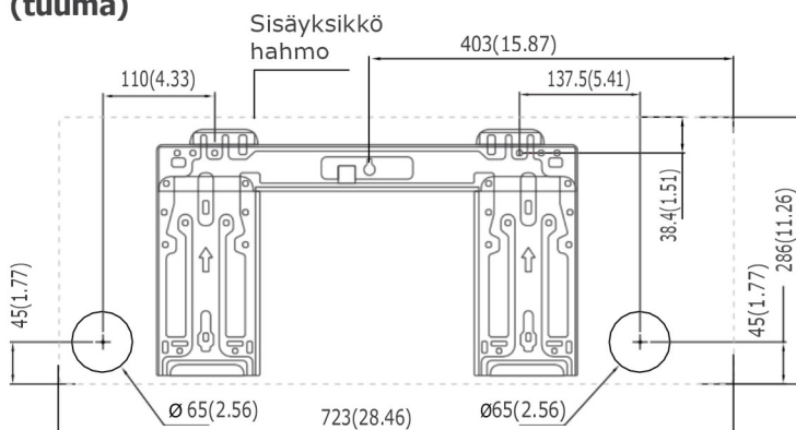
Malli A
