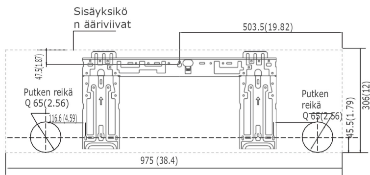
Malli C
