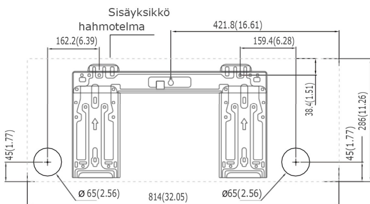
Malli B
